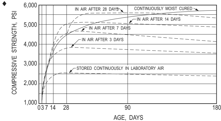
Concrete compressive strength varies with moist-curing conditions. Mixes tested had a water-cement ratio of 0.50, a slump of 3.5 in., cement content of 556 lb/yd 3 , and sand content of 36%, and air content of 4%.
